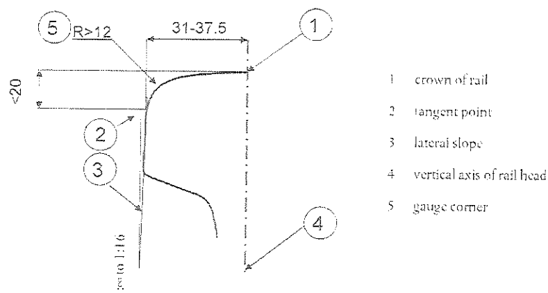
Railhead profile
