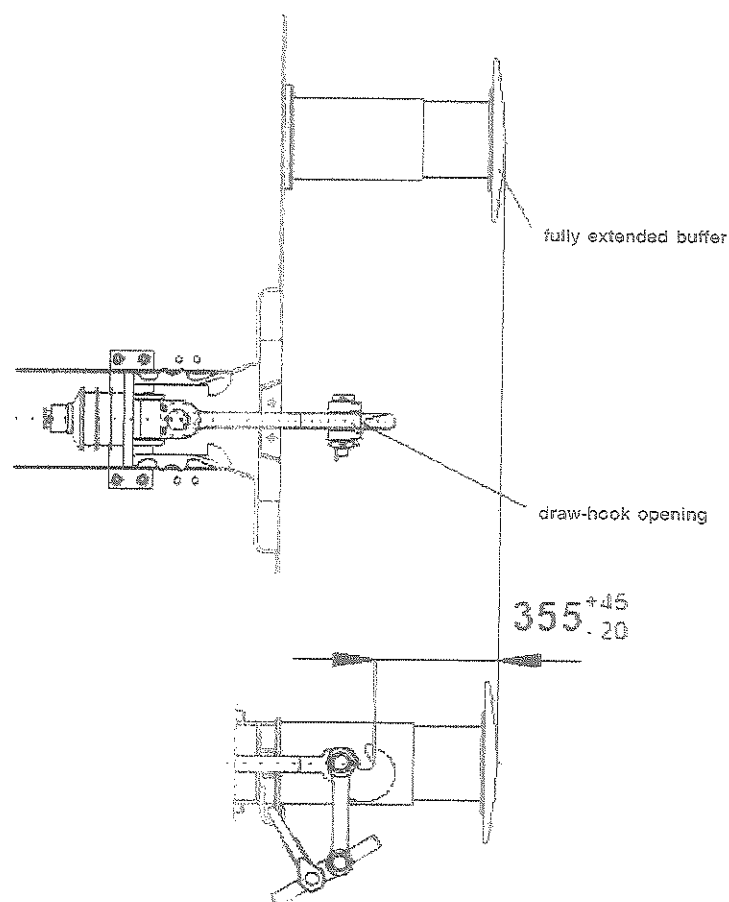
Figure C.1 Configuration of buffers and draw gear
