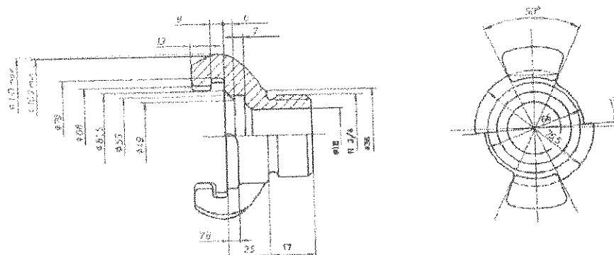
Figure A II1 The water filling adapters
