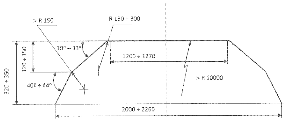
Fig. Configuration and dimensions of contact skates
